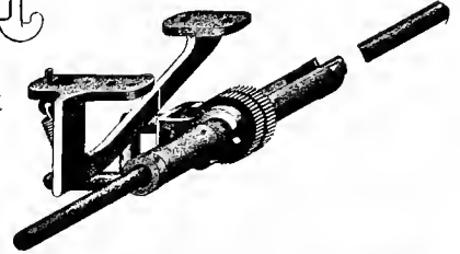
Fig. 1768. View of Adjuster, with Dust Proof Case removed to show Ratchet.
